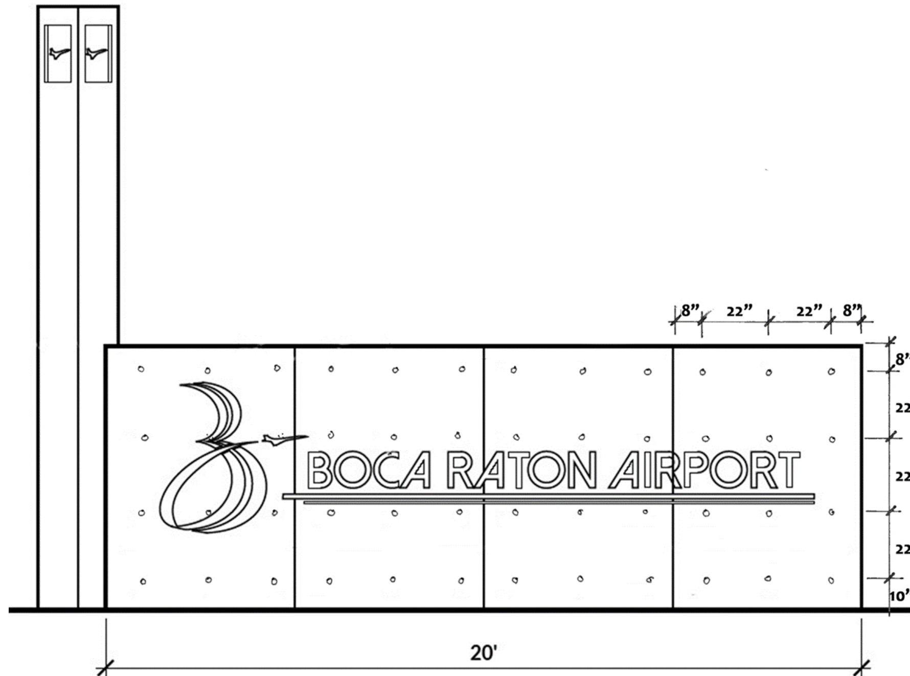
North Monument Sign Elevation - Snap Tie Layout
